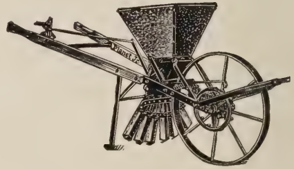
NO. 220 FERTILIZER DRILL
